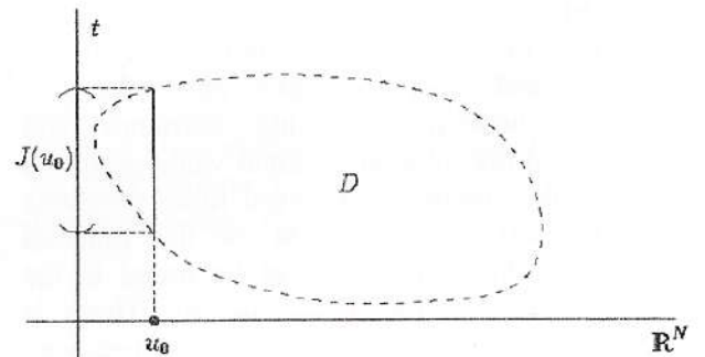
FIGURE 1 Dynamical systems and differential equations Domain of definition of the solution of (2.2)
