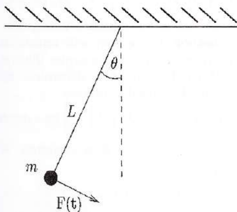
Dynamical systems and differential equations Forced pendulum
