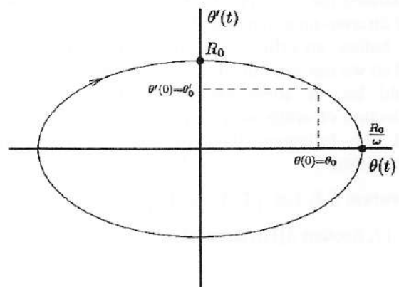
FIGURE 3 Dynamical systems and differential equations Orbit of the pendulum system
